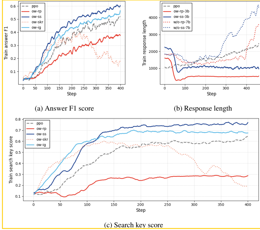
Figure 6: Training dynamics of correctness, response length, and search-key scores in ablation experiments. ‘w/o’ represent ‘with out’ while ‘ow’ for ‘only with’. ‘rp’ stands for ‘redundancy penalty’, ‘ig’ for ‘information gain’, ‘ss’ is ‘step score’ (‘ig’ + ‘rp’) and ‘skr’ means the global reward ‘search key reward’.
