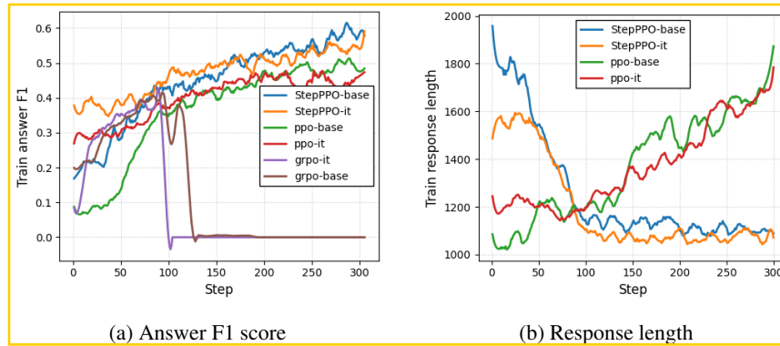
Figure 5: Comparison of StePPO vs. PPO.
