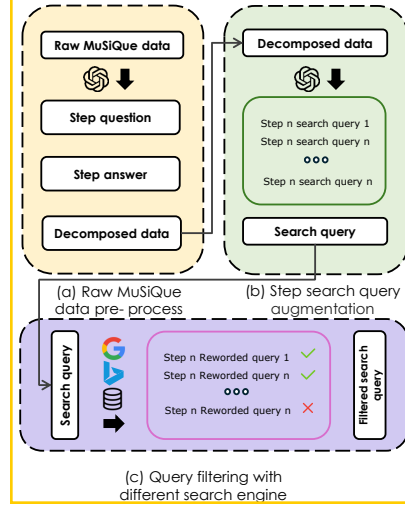
Figure 3: Data pipeline for generating the corresponding search query for the Q&A intermediate process.
